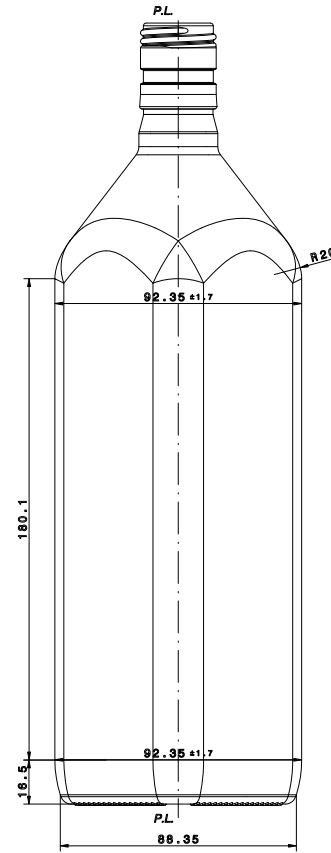
View through parting line
