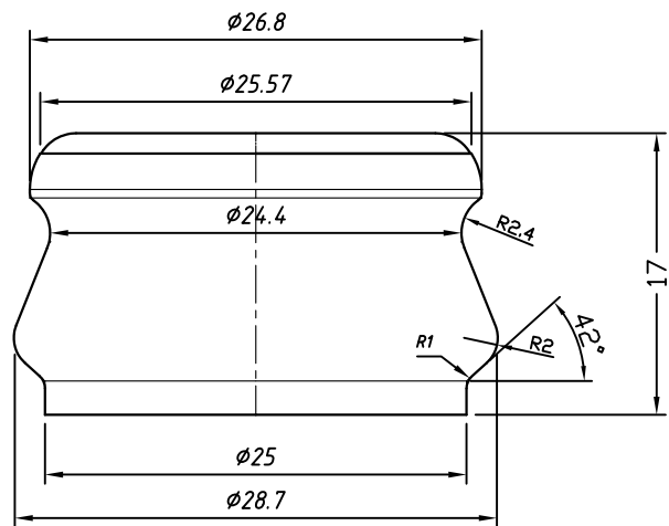
FINISH DETAIL
